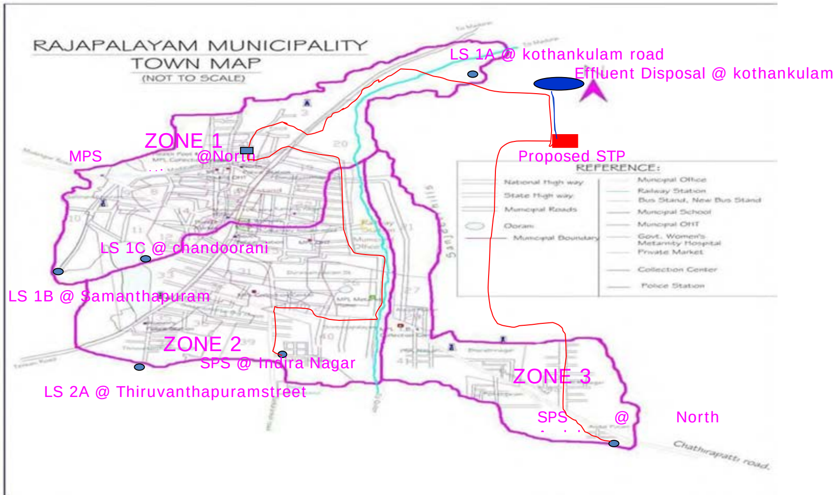
Figure 2: Proposed Sewerage Zones
