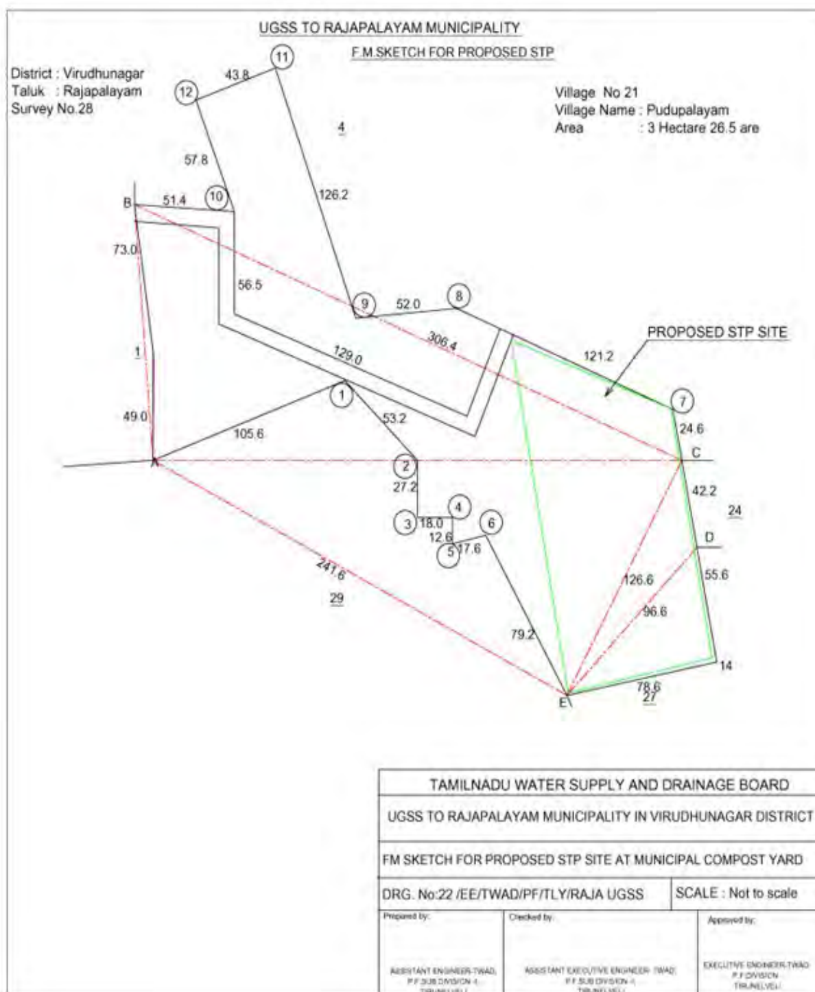
Figure 8: Sewage Treatment Plant Site Map
